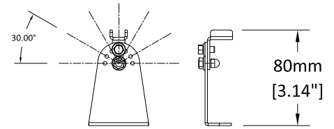
Wall Mount Bracket (Order Separately)
