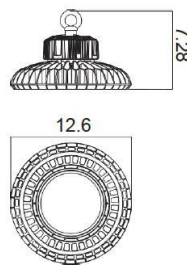
100-150W Dimension
