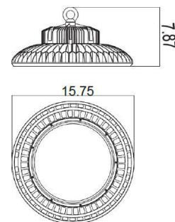
200-240W Dimension
